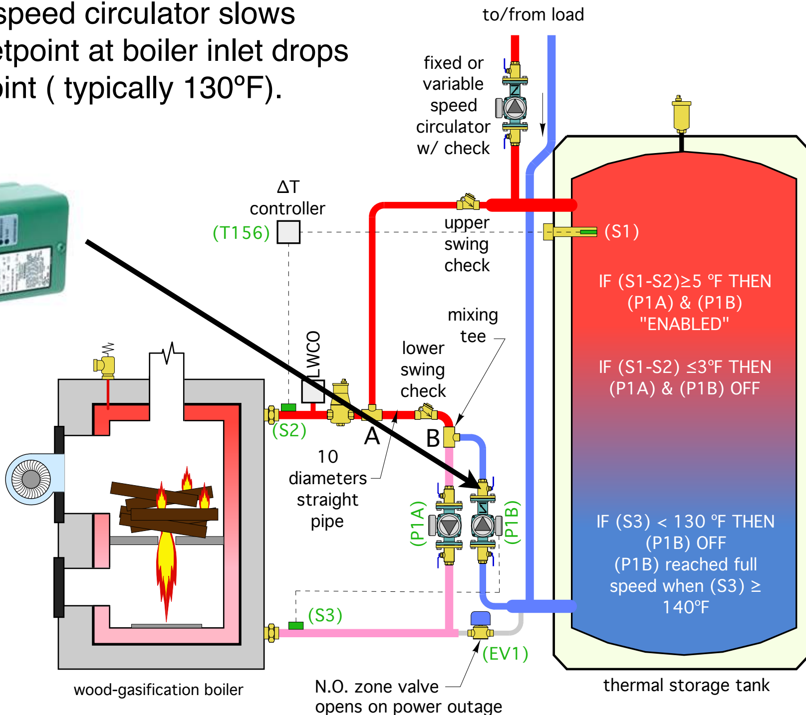
Taco 00-VS temperature controlled circulator
