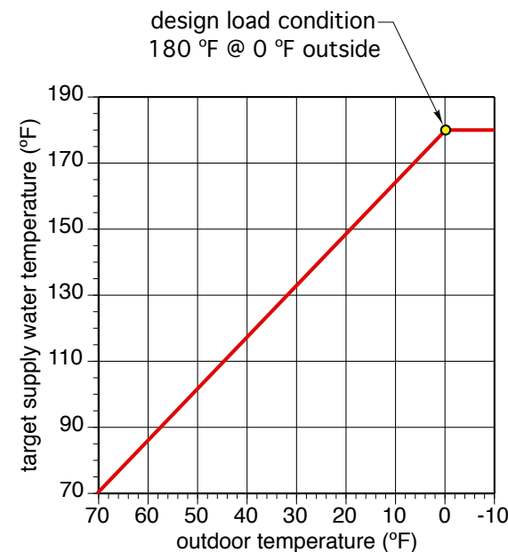
mixing reset control
