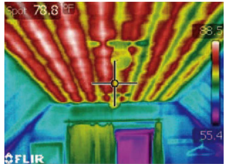
Thermal image of radiant ceiling in operation
