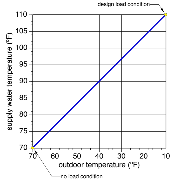
outdoor reset control setting for 3-way motorized mixing valve
