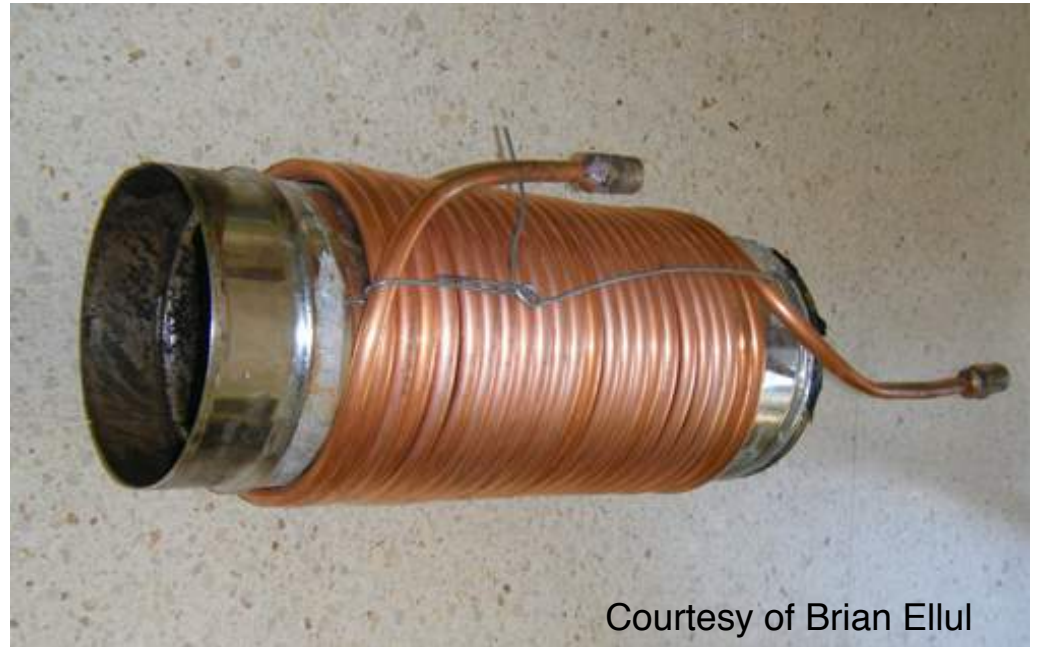
water jacket for stove pipe flue
