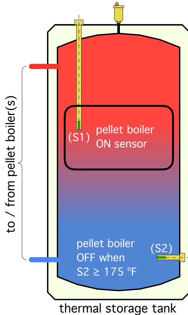
pellet boiler "start" condition
