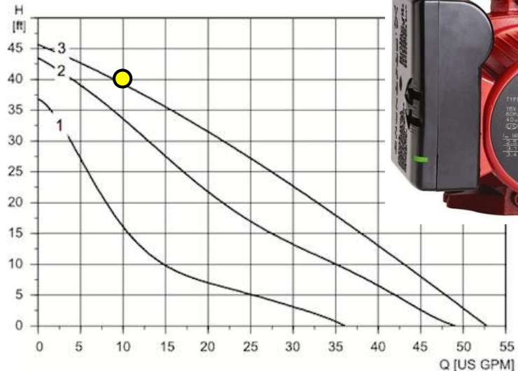
published pump curves for Grundfos UPS 26-150
