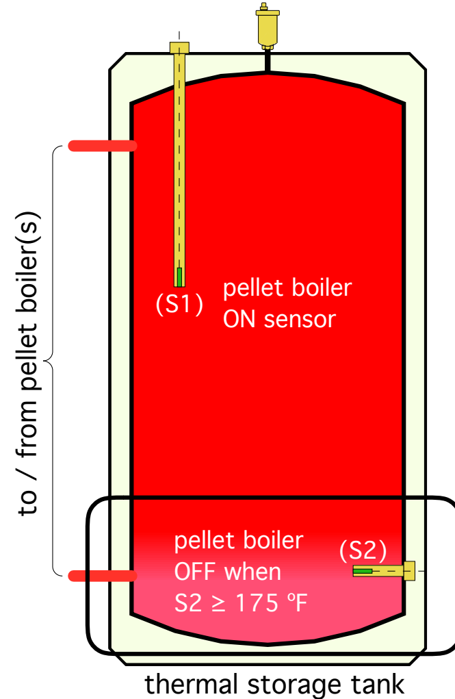
pellet boiler "stop" condition
