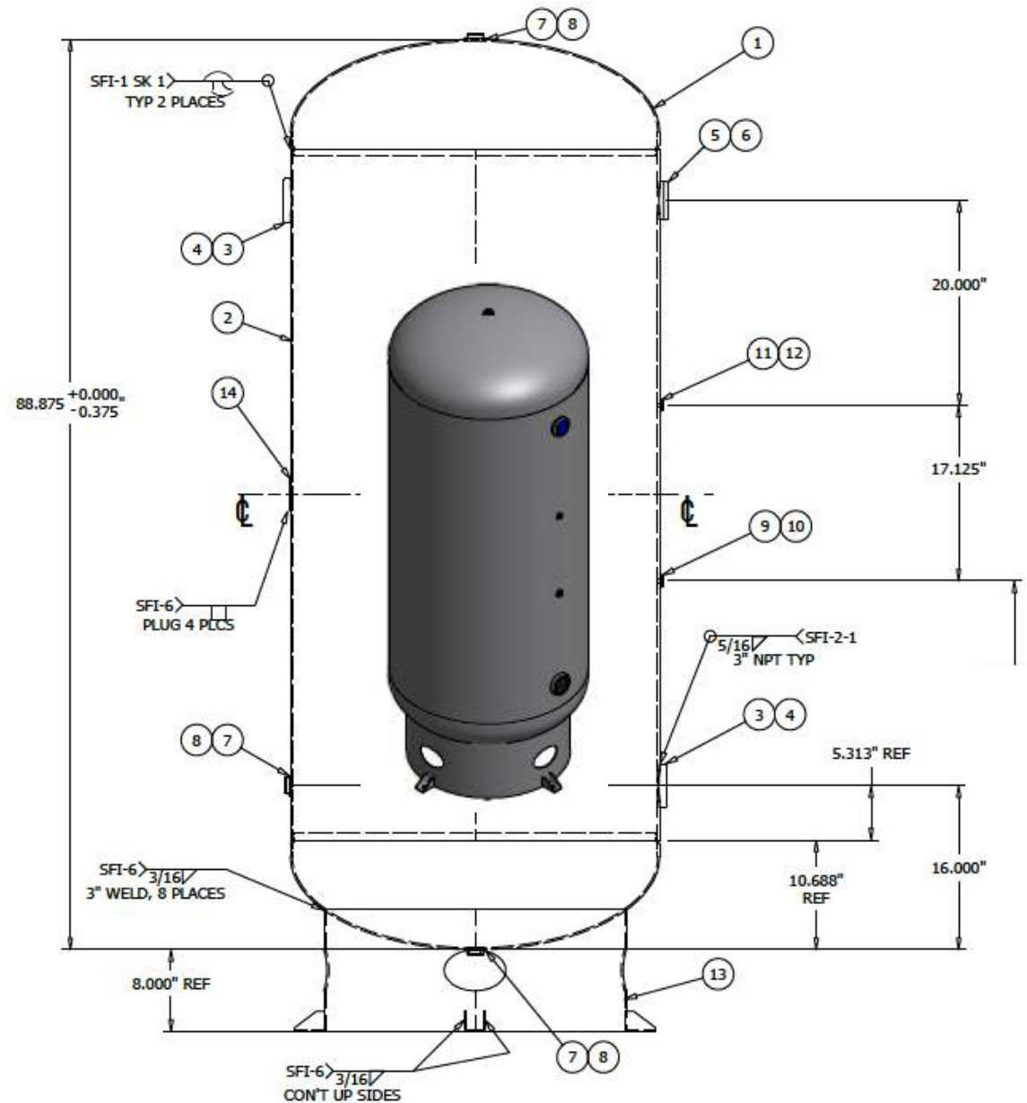
Alternate Heating of North America 400 gallon, ASME
