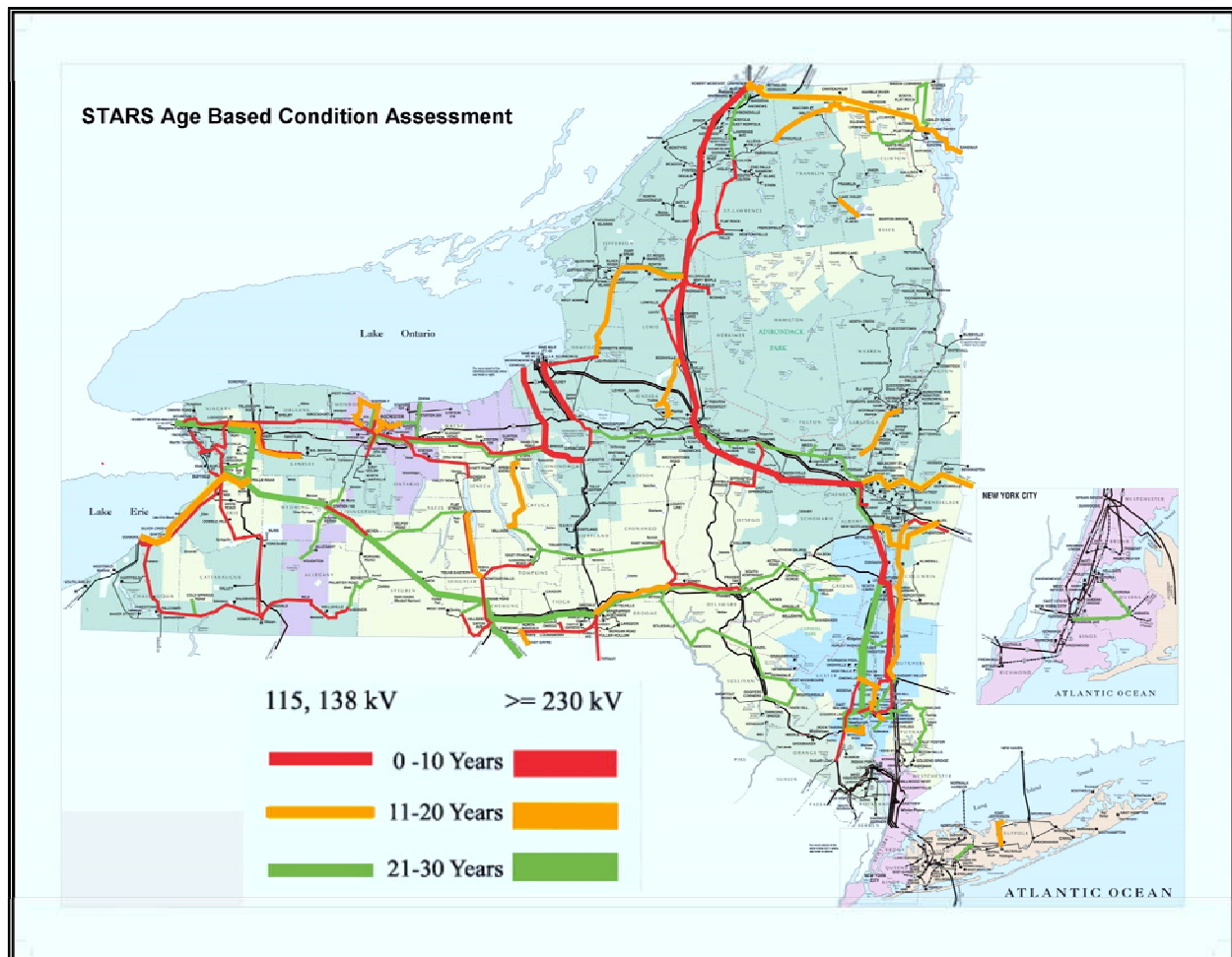
Figure 19. New York State Transmission Age Condition Assessment
