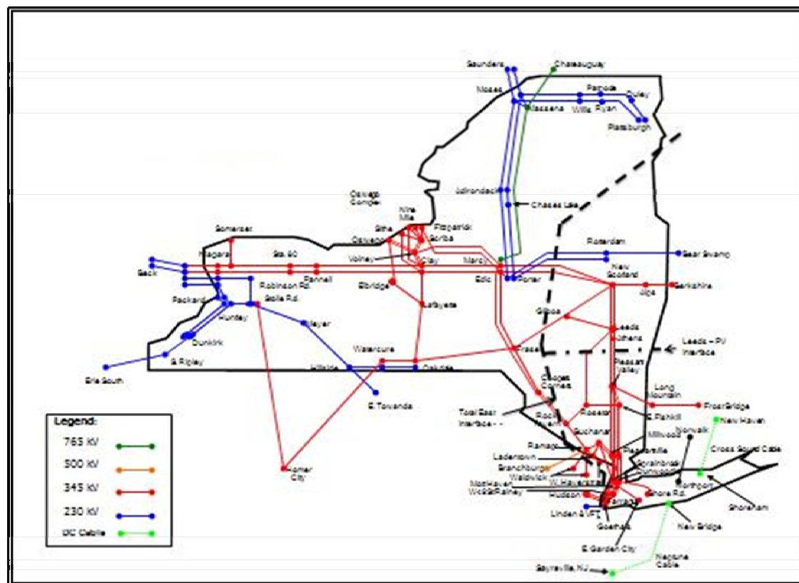
Figure 2. New York Control Area Transmission 230 kV and Above
