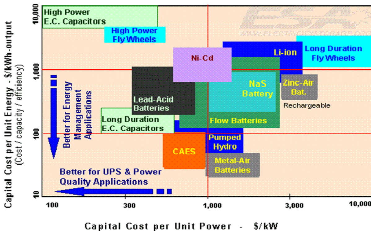
Figure 66 Capital cost per unit energy vs. per unit power (Energy Storage Association)
