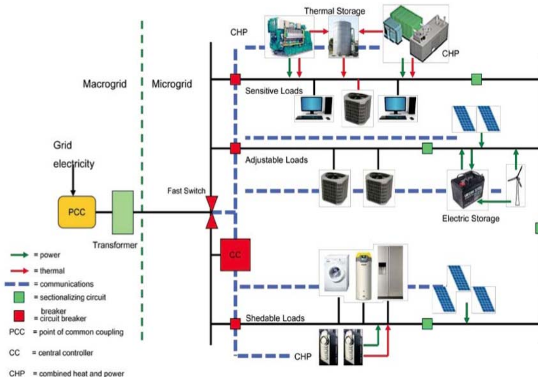
Figure 69 Micro-grid schematic 4
