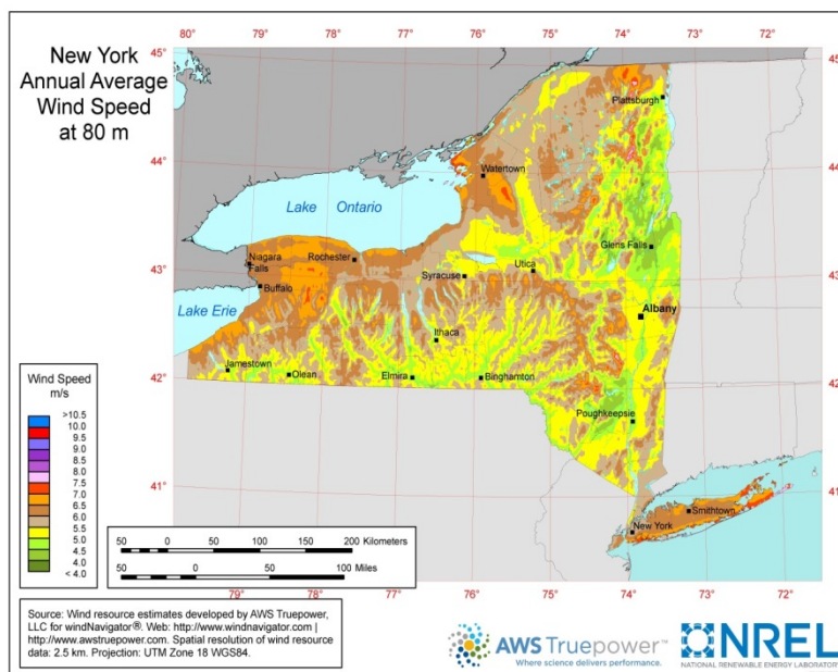
Figure 32 Wind resource map of New York State
