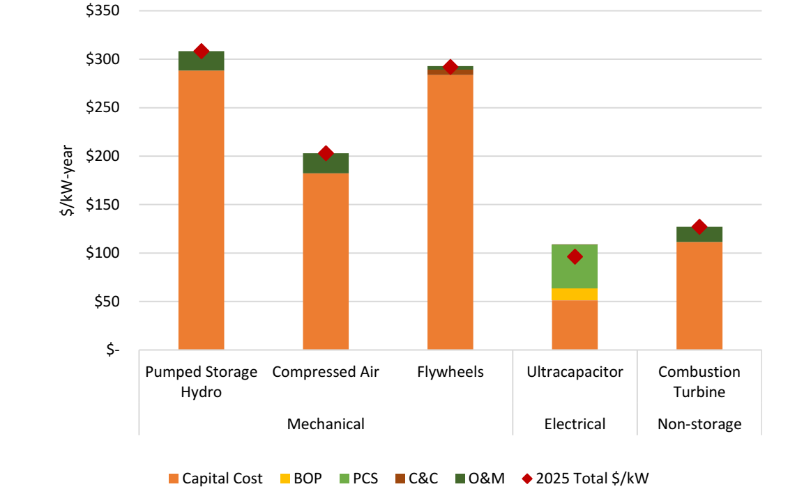
Figure 5.4. Annualized $/kW cost of non-battery technologies.
