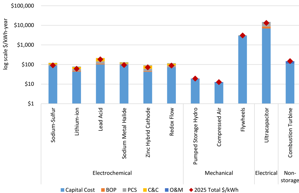
Figure 5.6. Annualized $/kWh cost of all technologies.
