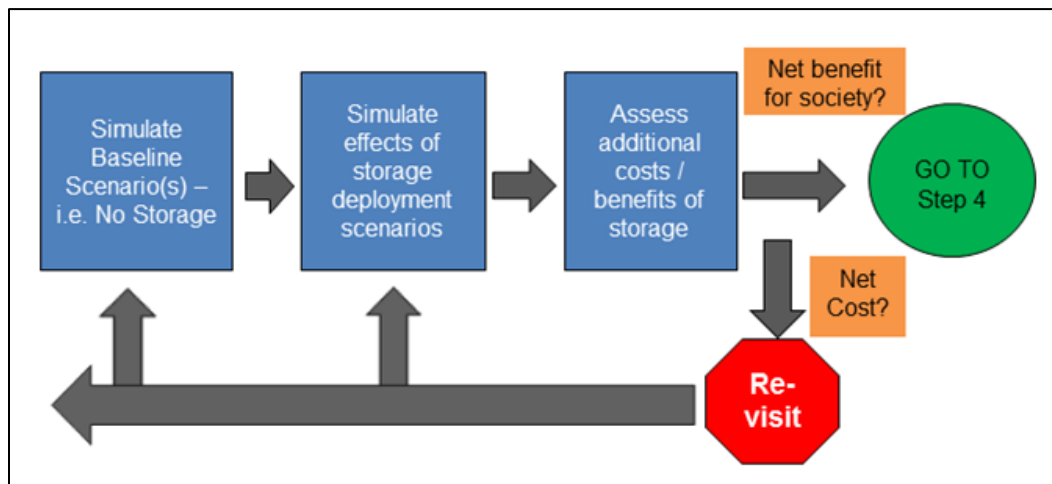
Figure 120. Decision Diagram for Step 3: Grid Impacts and Incidental Benefits (Source: EPRI)
