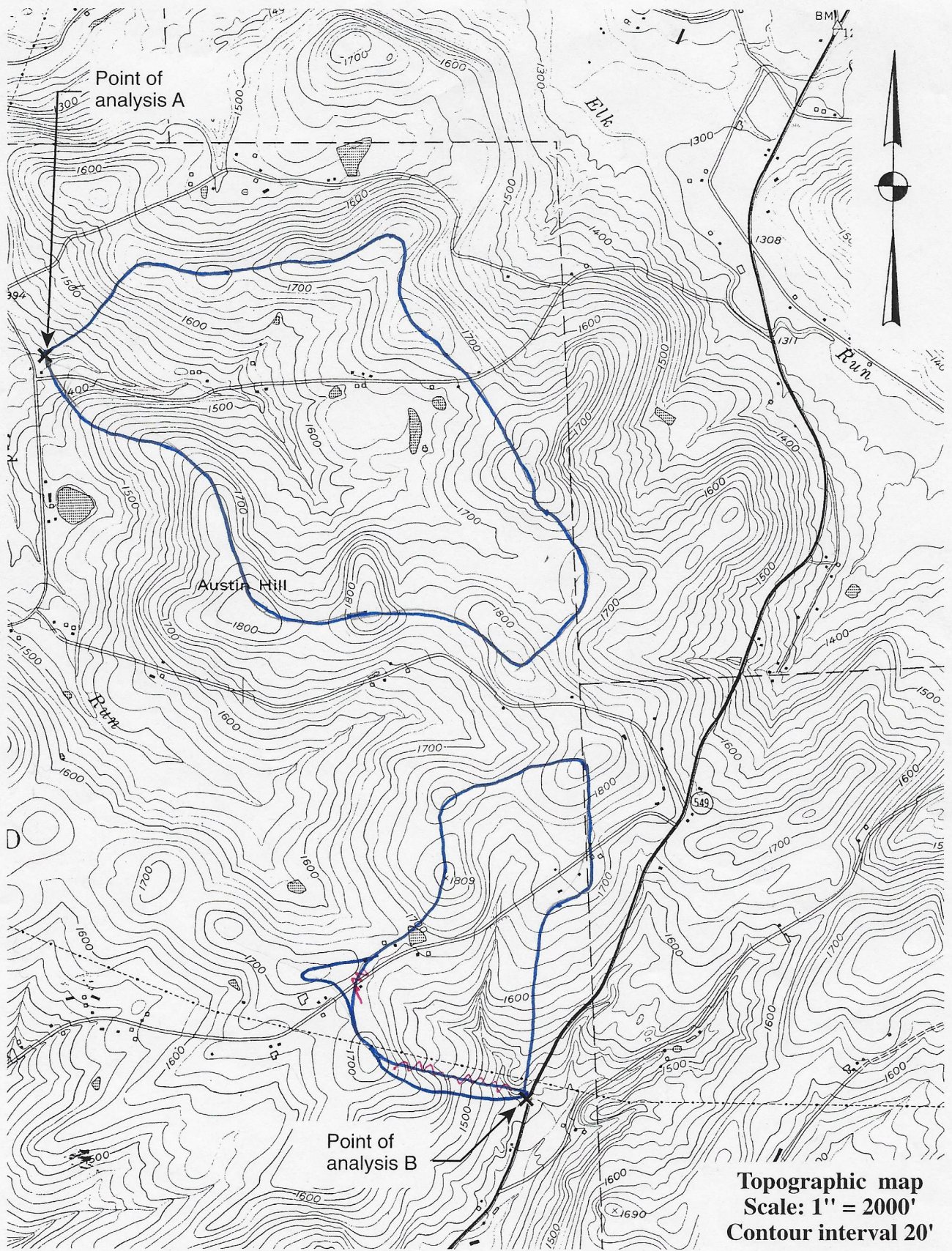
FIGURE 10-27 Topographic map for problem 8.
