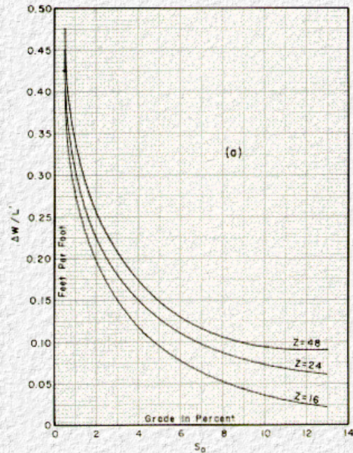
Figure 5-29. (a) & (b) P-1 7/8" Parallel Bar Grate
