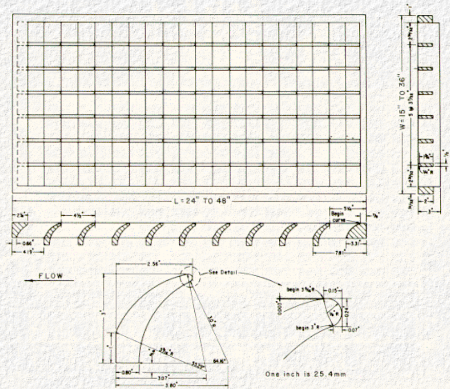
Figure 5-18. Curved Vane Grate
