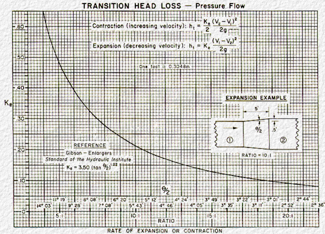
Figure 5-36. Transition Head Loss - Pressure Flow (from Los Angeles Standards)
