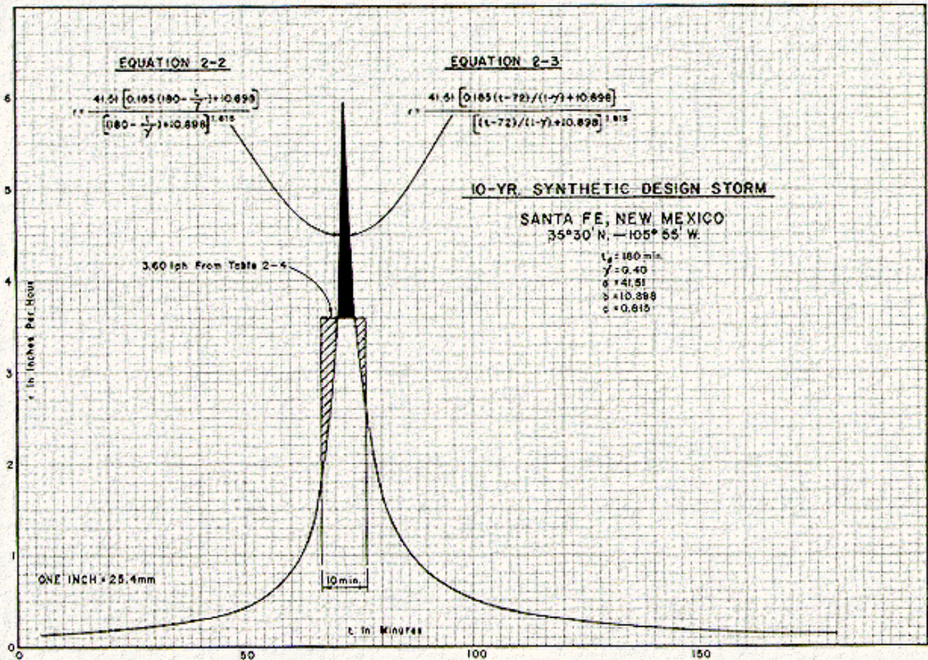
Figure 2-13. 10-Year Synthetic Design Storm
