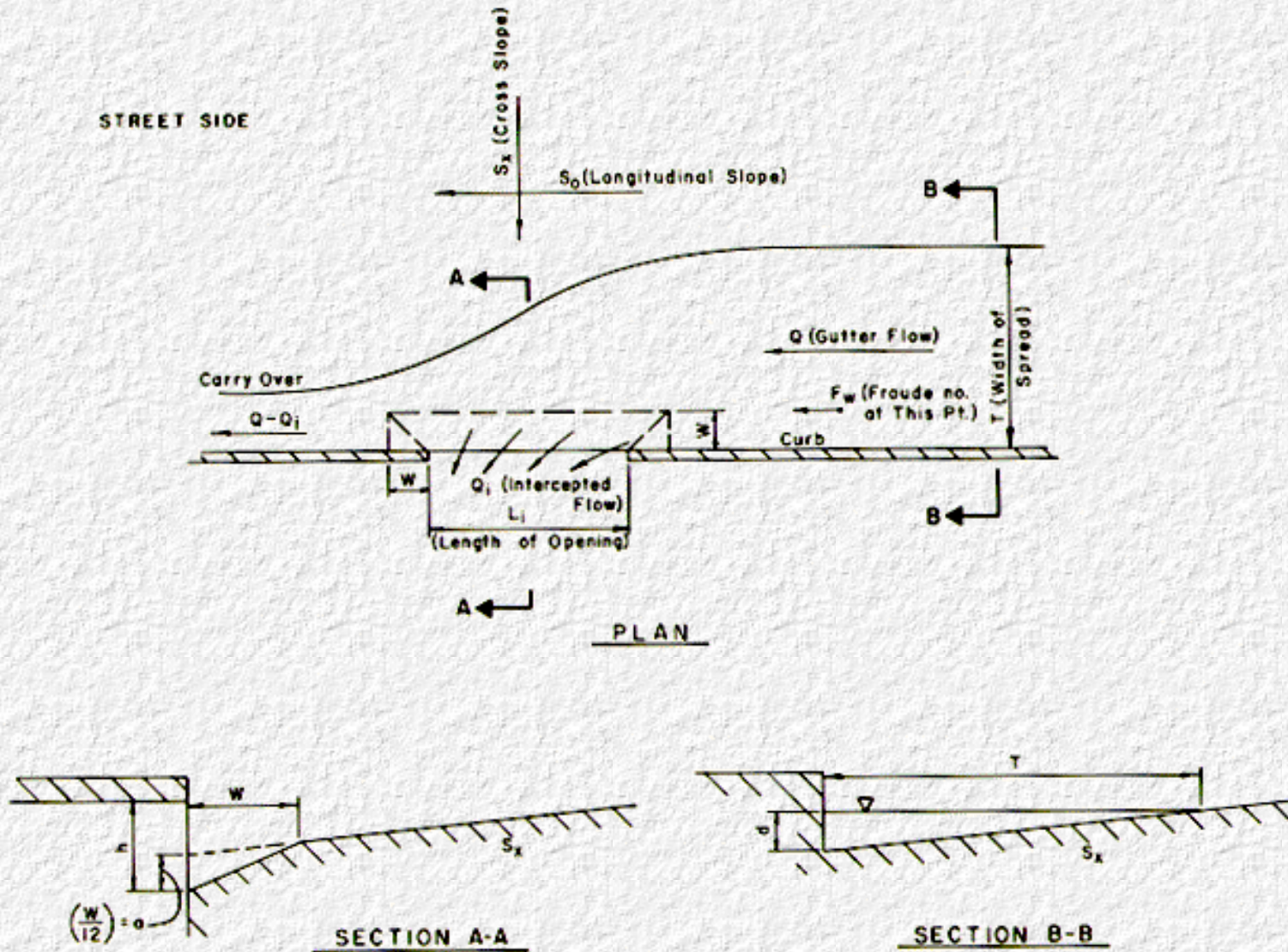
Figure 5-4. Graphical Definition of Symbols
