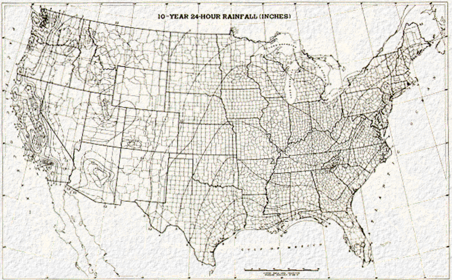
Figure 2-5. 10-Year 24-Hour Rainfall (Inches) (after National Weather Service)
