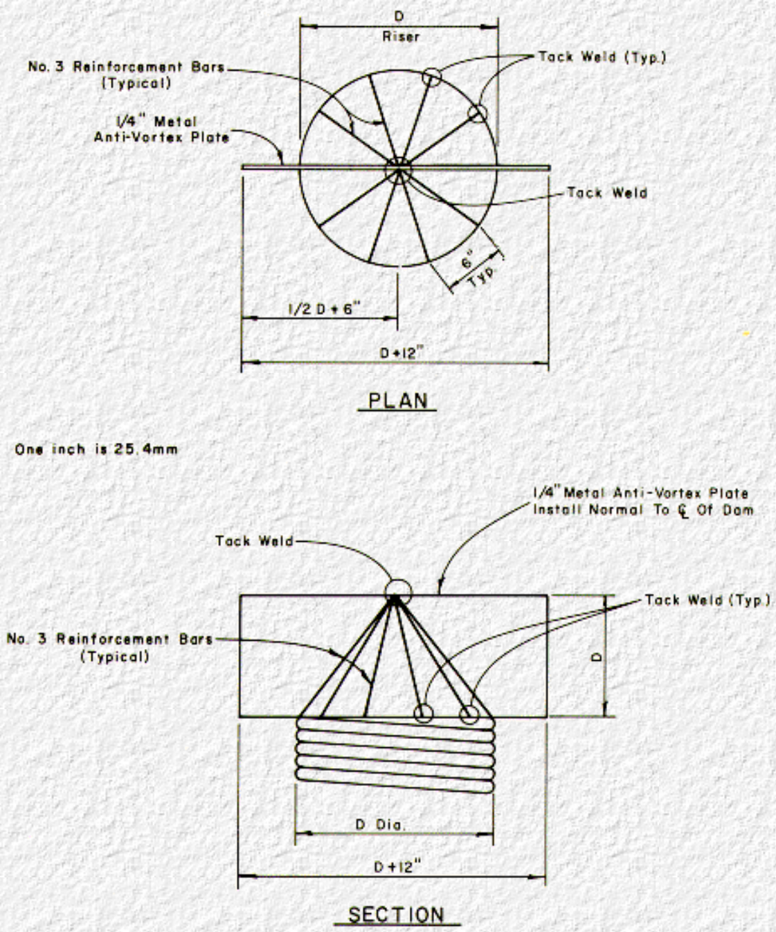
Figure 4-2(b). Detail of Trash Rack and Anti-Vortex Device
