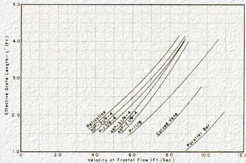
Figure 5-31. Minimum Effective Grate Length (Without Splashing)
