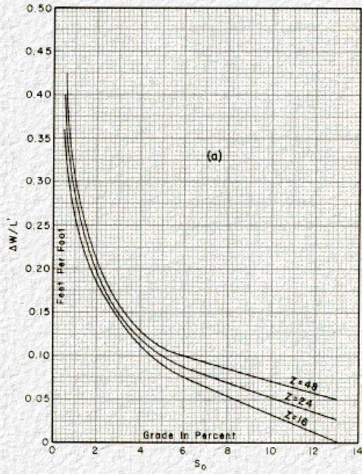
Figure 5-28. (a) & (b) P-1 1/8" Grate
