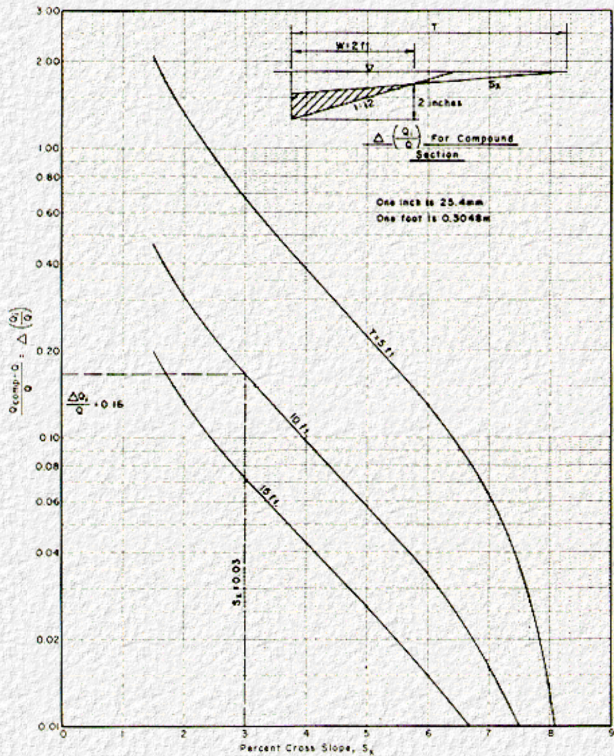
FIG. 5-8 Graph to give increment of discharge \Delta \left( \frac{Q}{Q} \right) for composite section
