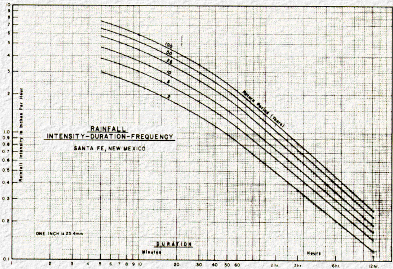
Figure 2-9. Rainfall Intensity-Duration-Frequency (Santa Fe, New Mexico)
