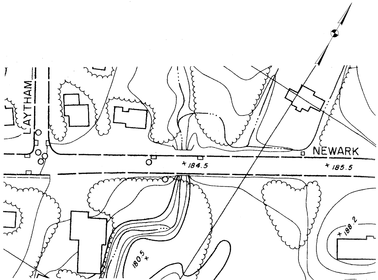
FIGURE 13-27 ROAD PLAN AND PROFILE SHOWING EXISTING BOX CULVERT FOR PROBLEM 4.
