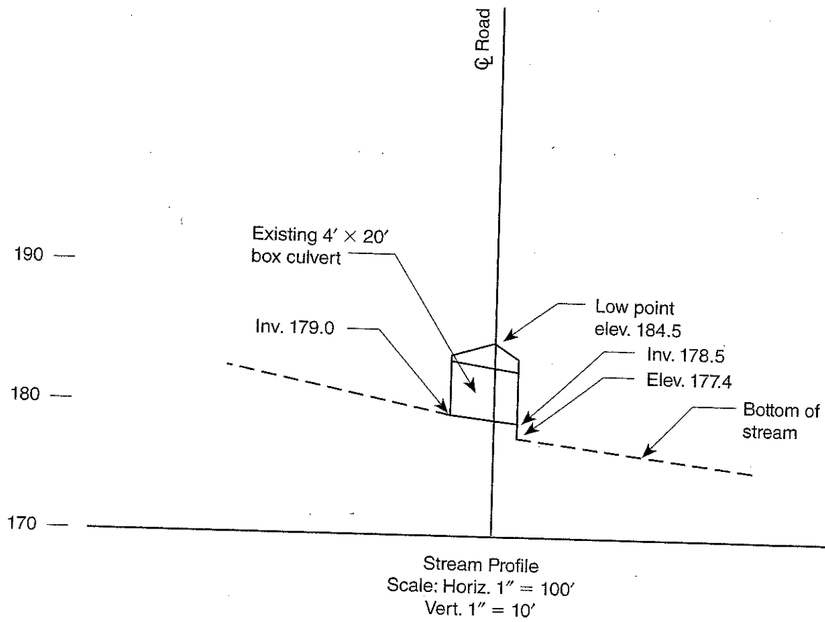
FIGURE 13-28 STREAM PROFILE SHOWING EXISTING CULVERT FOR PROBLEM 4.
