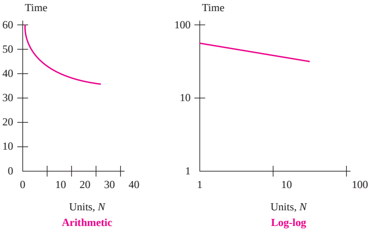
FIGURE 11.3 Plots of time estimates for a learning rate of 90% for 32 units with T_1 = 60 minutes.
