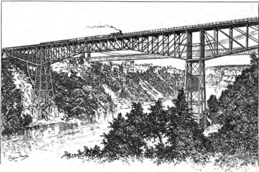
The Niagara Cantilever Bridge Completed.
