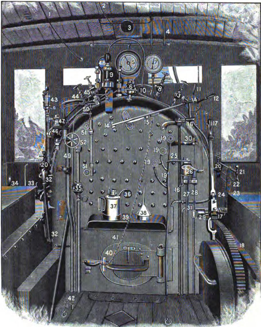
Fig. 35.—Cab End of a Locomotive and its Attachments.
