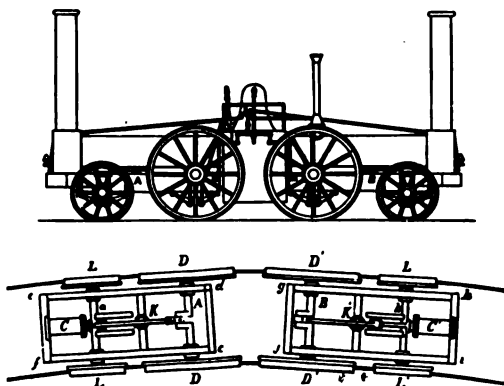
Fig. 5.—"South Carolina," 1831, and Plan of its Running Gear.
