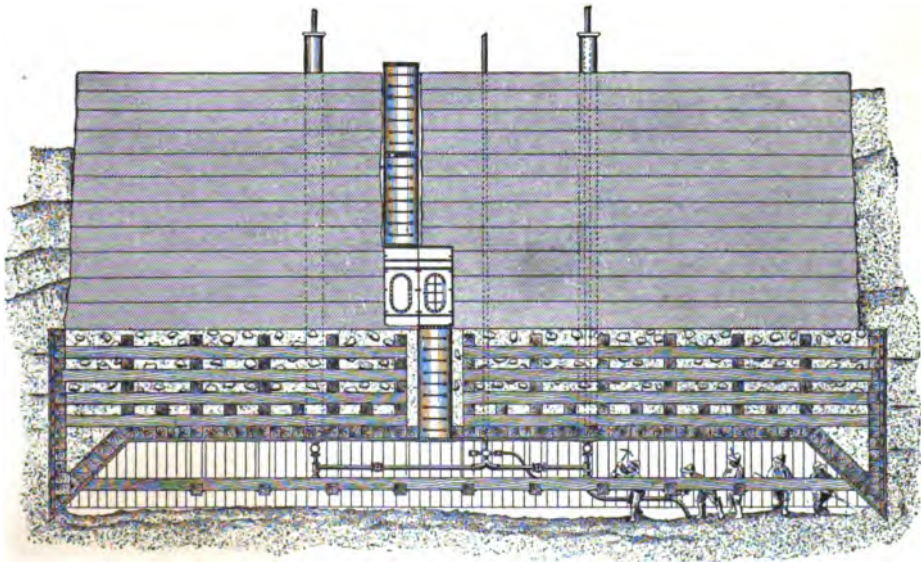
Transverse Section of Pneumatic Caisson.
