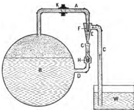
Fig. 18.—Rudimentary Injector.
