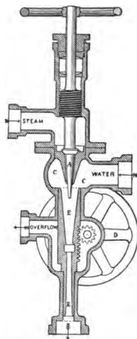
Fig. 19.—Injector used on Locomotives.
