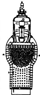
Fig. 17.—Transverse Section.
