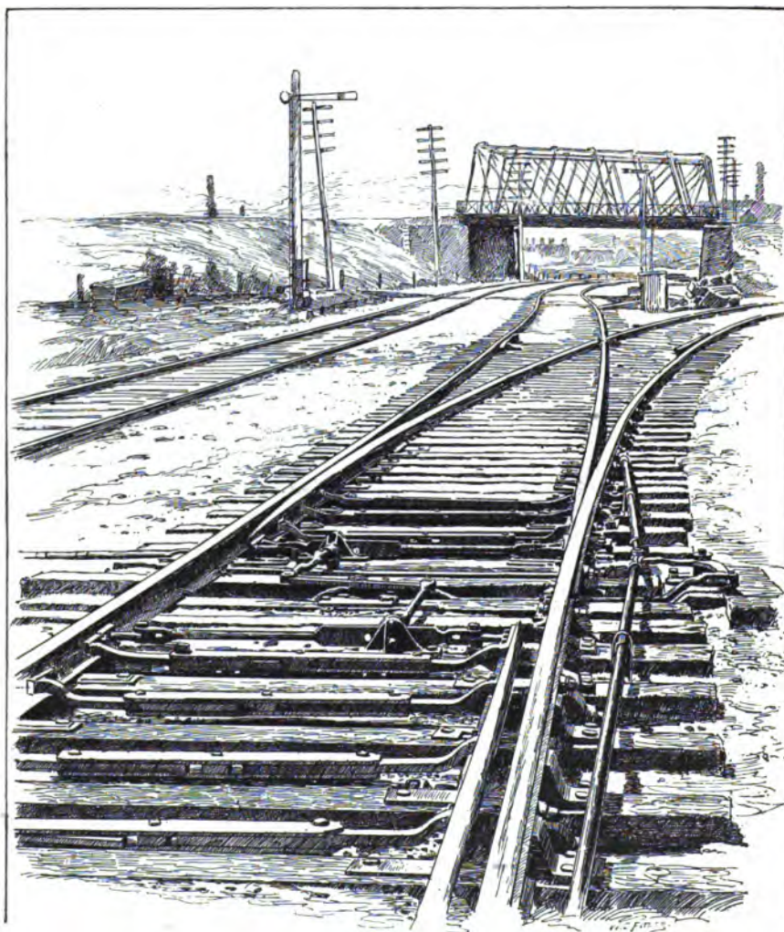
Split Switches with Facing-point Locks and Detector-bars.
