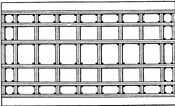
Foundation Crib of the Poughkeepsie Bridge.
