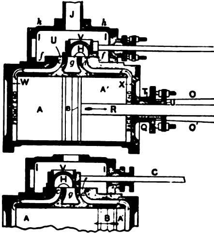
Fig. 20 (above) and 21.—Sections of a Locomotive Cylinder.
