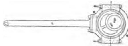
Fig. 23.—Eccentric and Strap.
