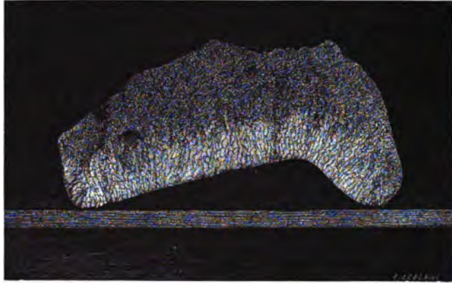
Fig. 52.—Section of the Tread and Flange of a Car Wheel.
