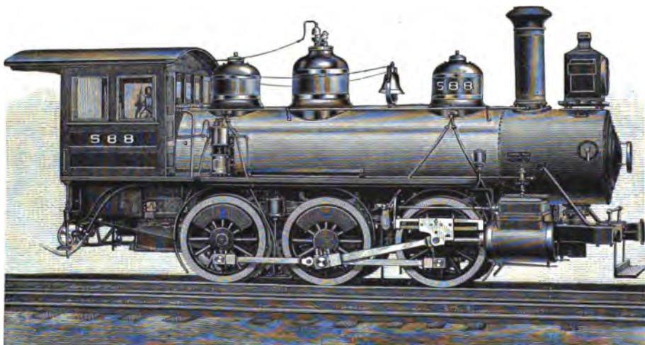
Fig. 26.—Six-wheeled Switching Locomotive. By the Schenectady Locomotive Works.
