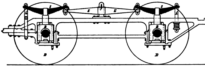
Fig. 15.—Driving Wheels, Frames, Spurs, etc., of American Locomotive.
