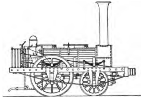
Fig. 8.—The "Planet."
