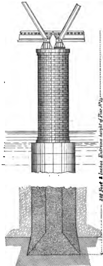
Pier of Hawkesbury Bridge, Australia.
